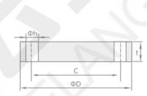
BL of nominal size 10A to 600A
