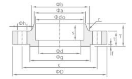
SW of nominal size 10A to 80A
